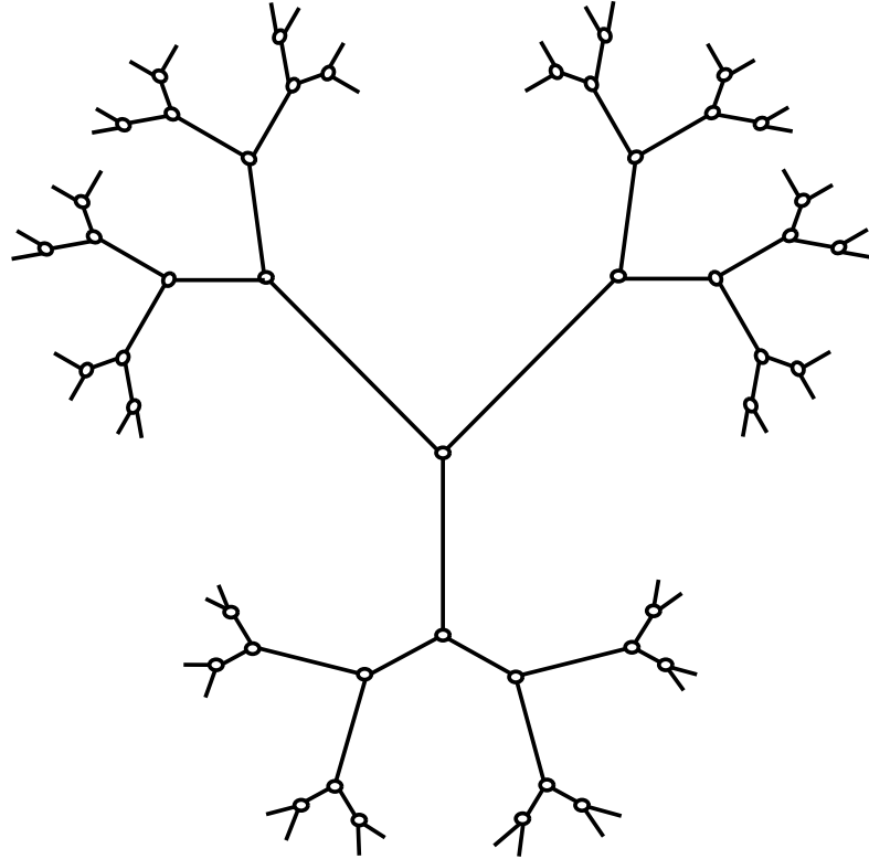
Figure 4 : Bruhat-Tits building of GL_2(K) , when |K| = 2 .
