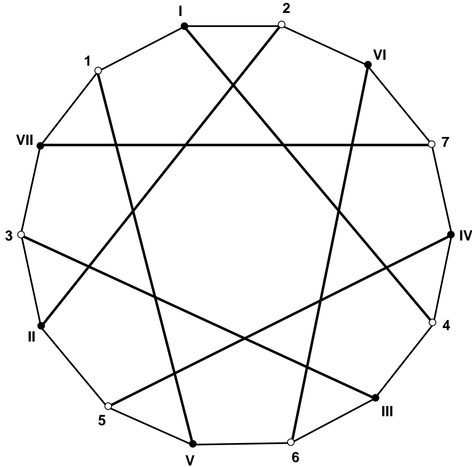
Figure 5 : Spherical Tits building of \mathrm{GL}_3(K) , when |K| = 2 .
